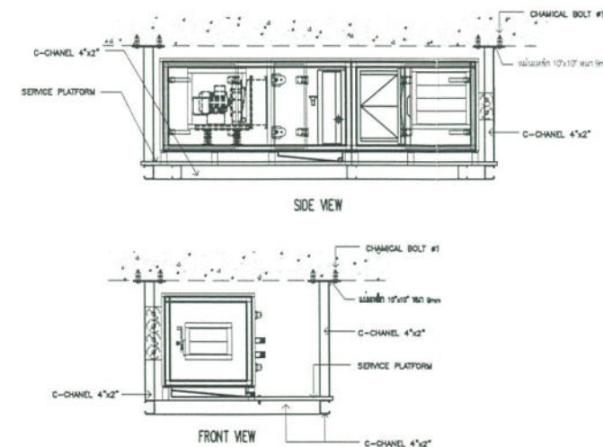
INSTALLATION SUPPORT AHU
