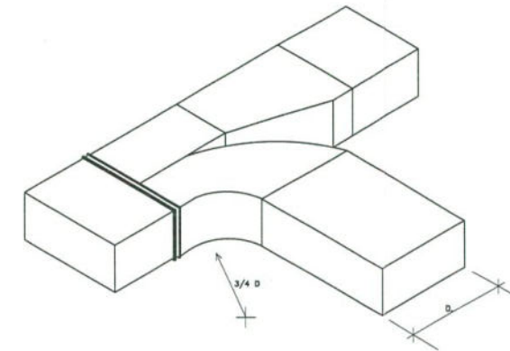
PARALLEL FLOW BRANCH.
